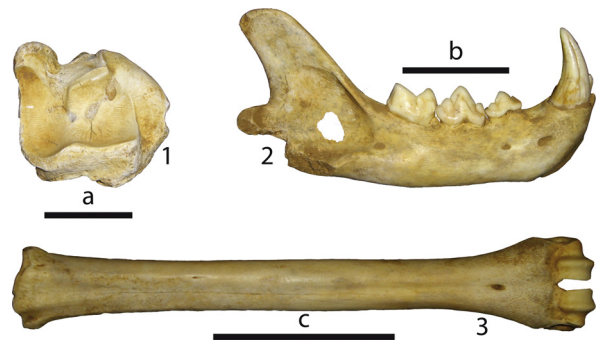
Fig. 3. 1: Bison priscus , left centrotarsal. 2: Panthera pardus , labial view of right mandible. 3: Rupicapra pyrenaica , right metatarsal. Scale bars = 5 cm, a for 1, b for 2 and c for 3.
